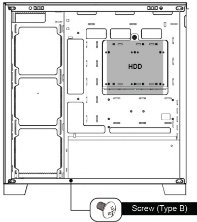
HDD Drive Installation
