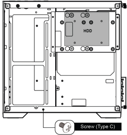
HDD Drive Installation
