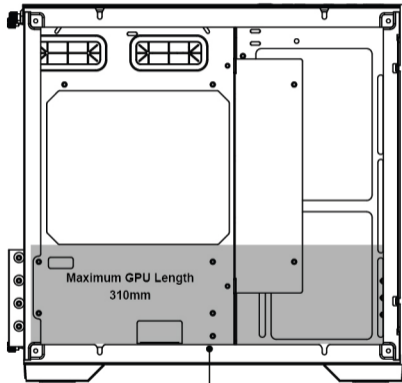
Graphics Processing Unit and other expansion cards
