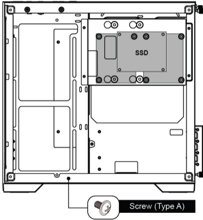
SSD Drive Installation
